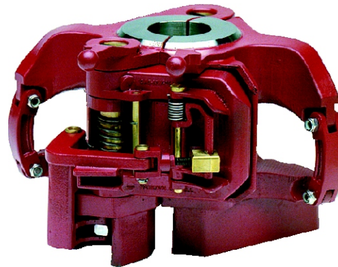
HGG Hydraulic Actuated Elevator
