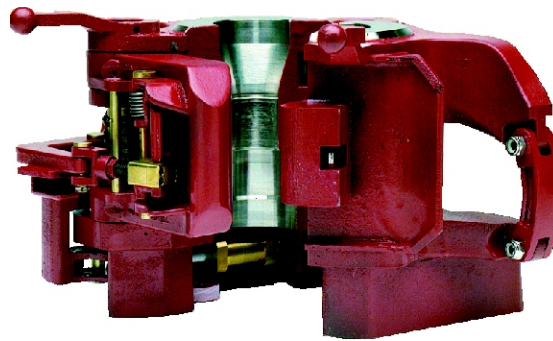
HGG Hydraulic Actuated Elevator with Wear Bushing Groove shown
